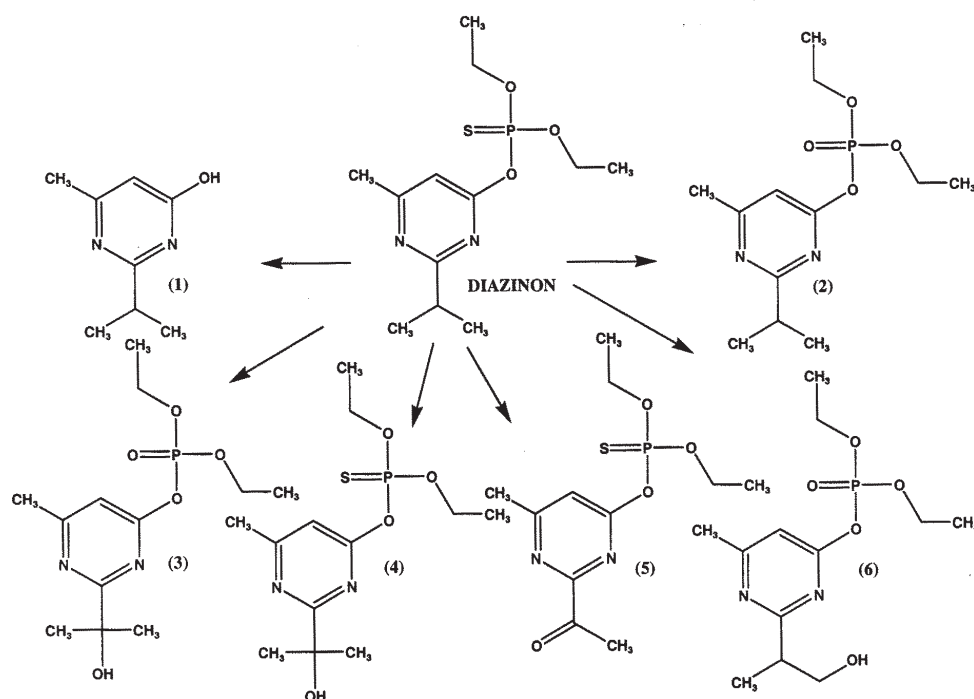
Scheme 1. Scheme of the proposed photodegradation pathway for diazinon: 2-isopropyl-6-methyl-pyrimidin-4-ol, (IMP) (1), diazoxon (2), hydroxydiazoxon (3), hydroxydiazinon (4) diazinon methyl ketone (5), 2-hydroxydiazoxon (6)
